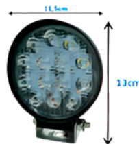
NEBLINERO LED 4.5" 32V 42W/6000K/2500 SF-5042-E SF50023
